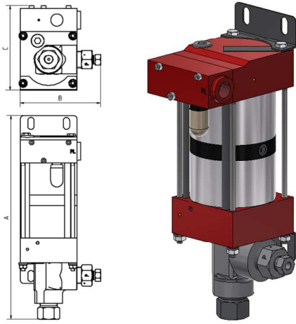
M189-2 (L) single acting, double air drive head (Standard= Bottom inlet)
